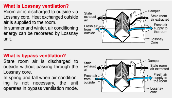
■ By-pass / Lossnay ventilation map in automatic ventilation mode
