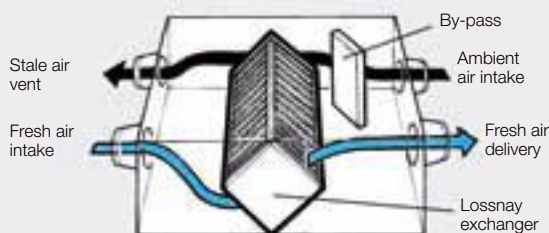
EXAMPLE OF BYPASS FUNCTION IN FREE-COOLING MODE
