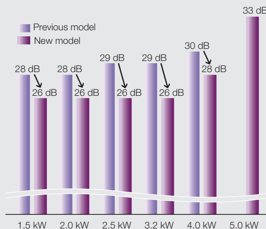
PLFY-P-VFM Cooling SLP [Lo]
